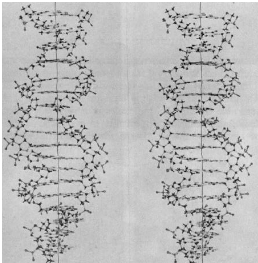
Figure 1. The original New Zealand SBS structure, as published in PNAS 1976 (ref. 1) – Courtesy the late Dr G. A. Rodley.
