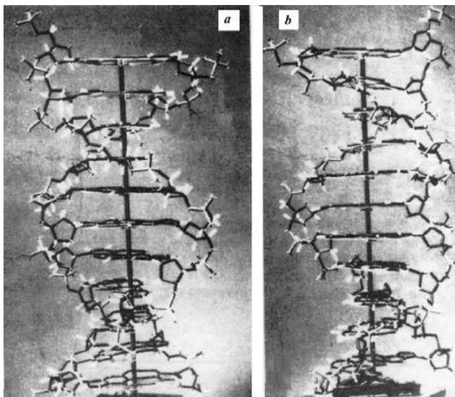
Figure 2. The original Indian SBS structure, as published in Current Science 1976 (ref. 2).
